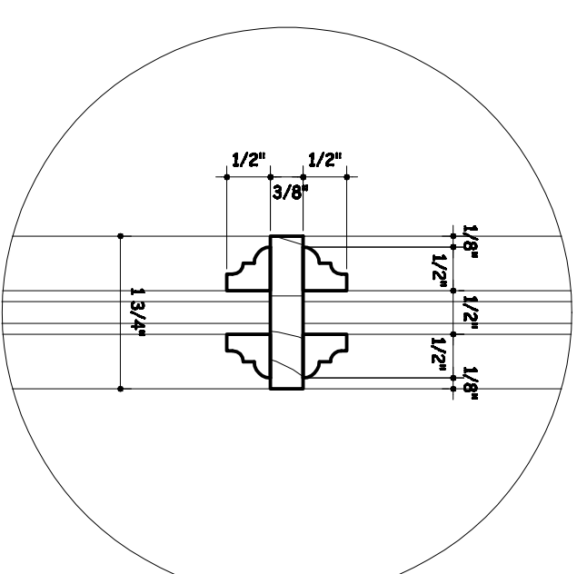
GRID FRAME DETAIL "D"
