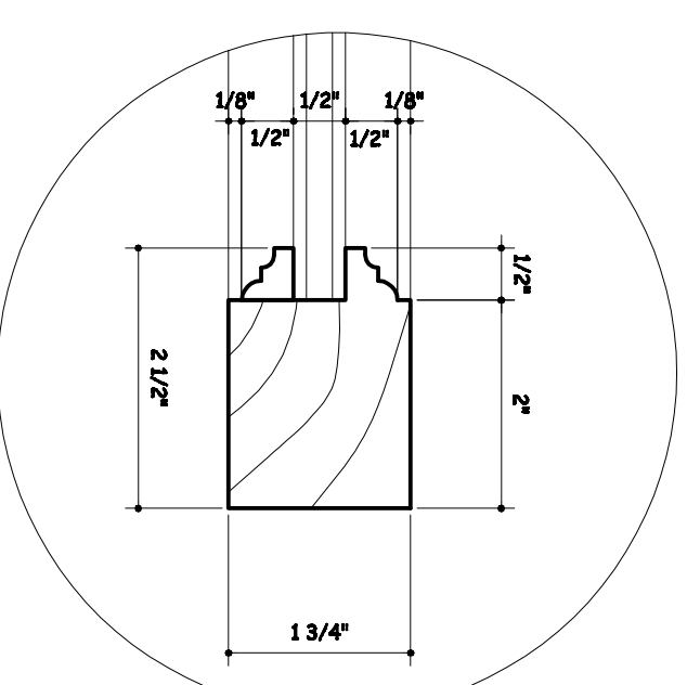
SIDE FRAME DETAIL "B"
