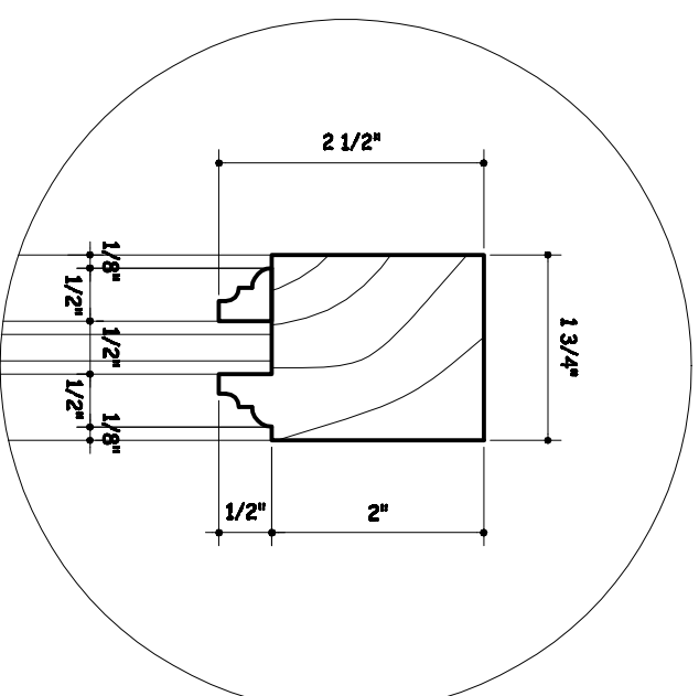
TOP FRAME DETAIL "C"
