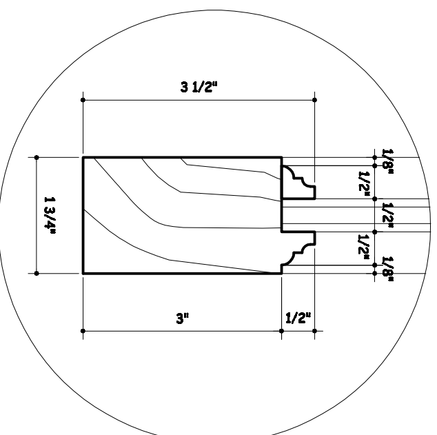
BOTTOM FRAME DETAIL "A"
