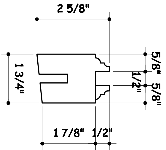
BOTTOM FRAME @ SLIDER
