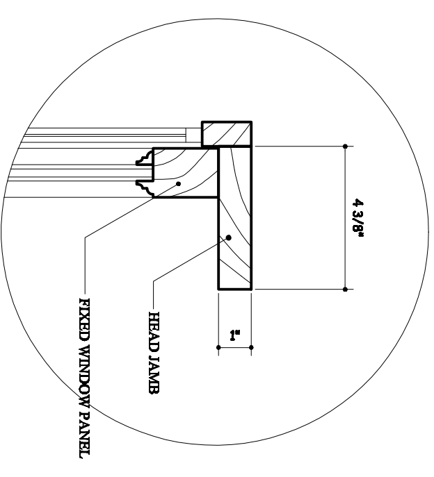
HEADER DETAIL "3"
