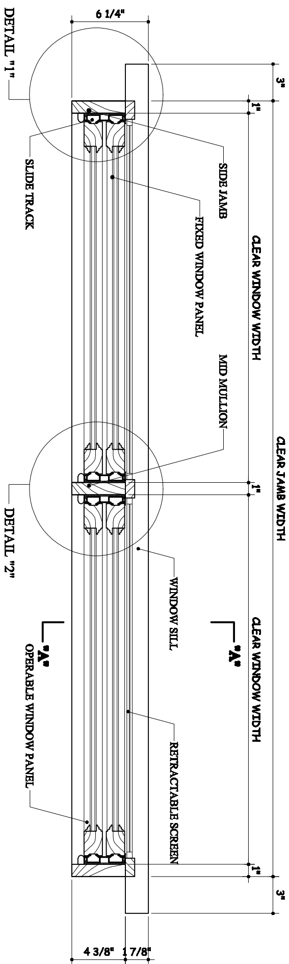
TOP VIEW
