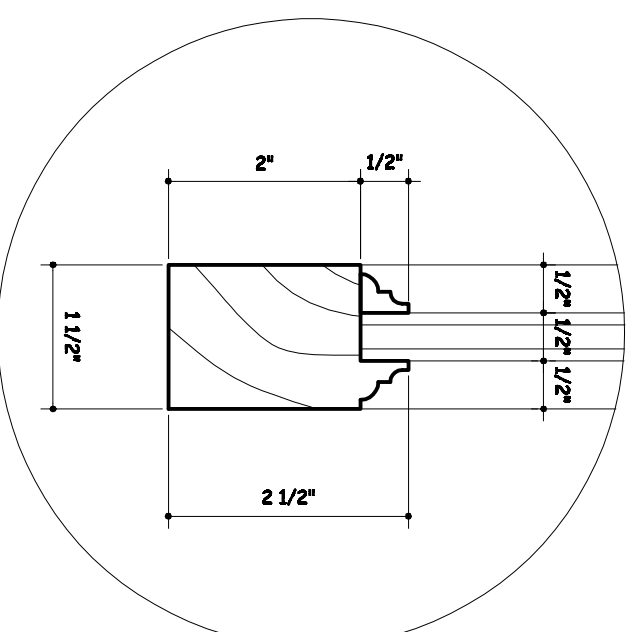
BOTTOM FRAME @ FIXED PANEL DETAIL "A-2"
