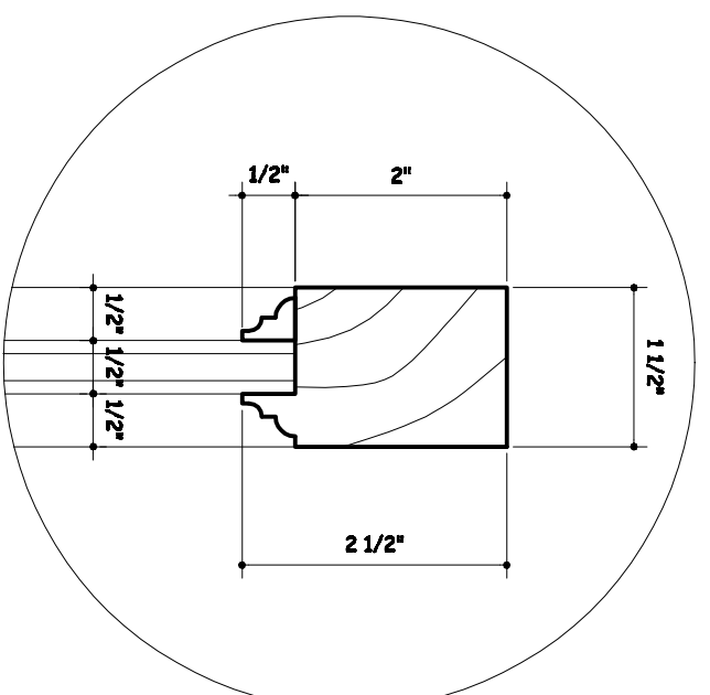
TOP FRAME DETAIL "C"
