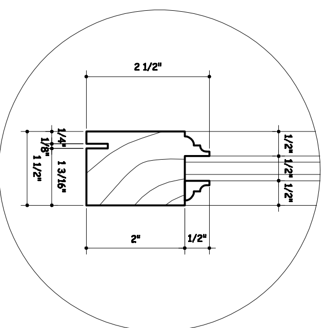
BOTTOM FRAME @ OPENABLE PANEL DETAIL "A-1"
